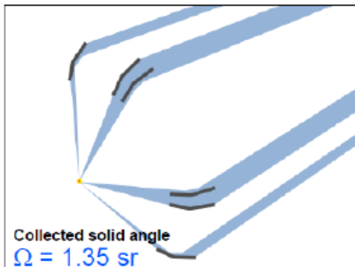
3-shell collector
