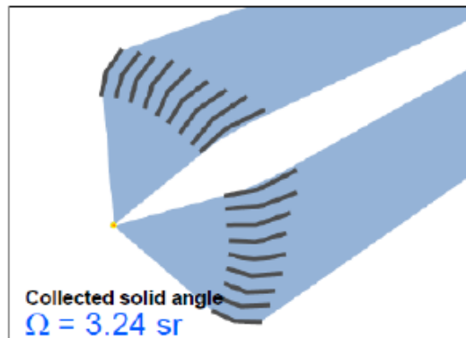
9-shell collector
